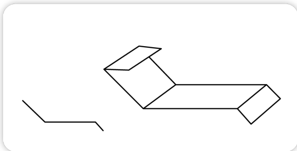
ANGLED APRON FLASHING
