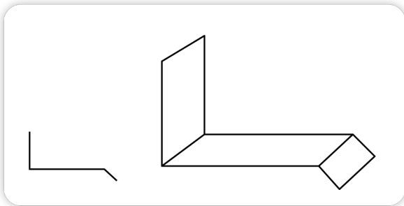
STANDARD APRON FLASHING
