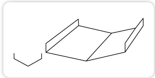
VALLEY GUTTER WITH UPSTAND
