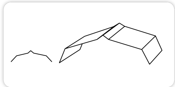
BIRDBEAK RIDGE CAPPING
